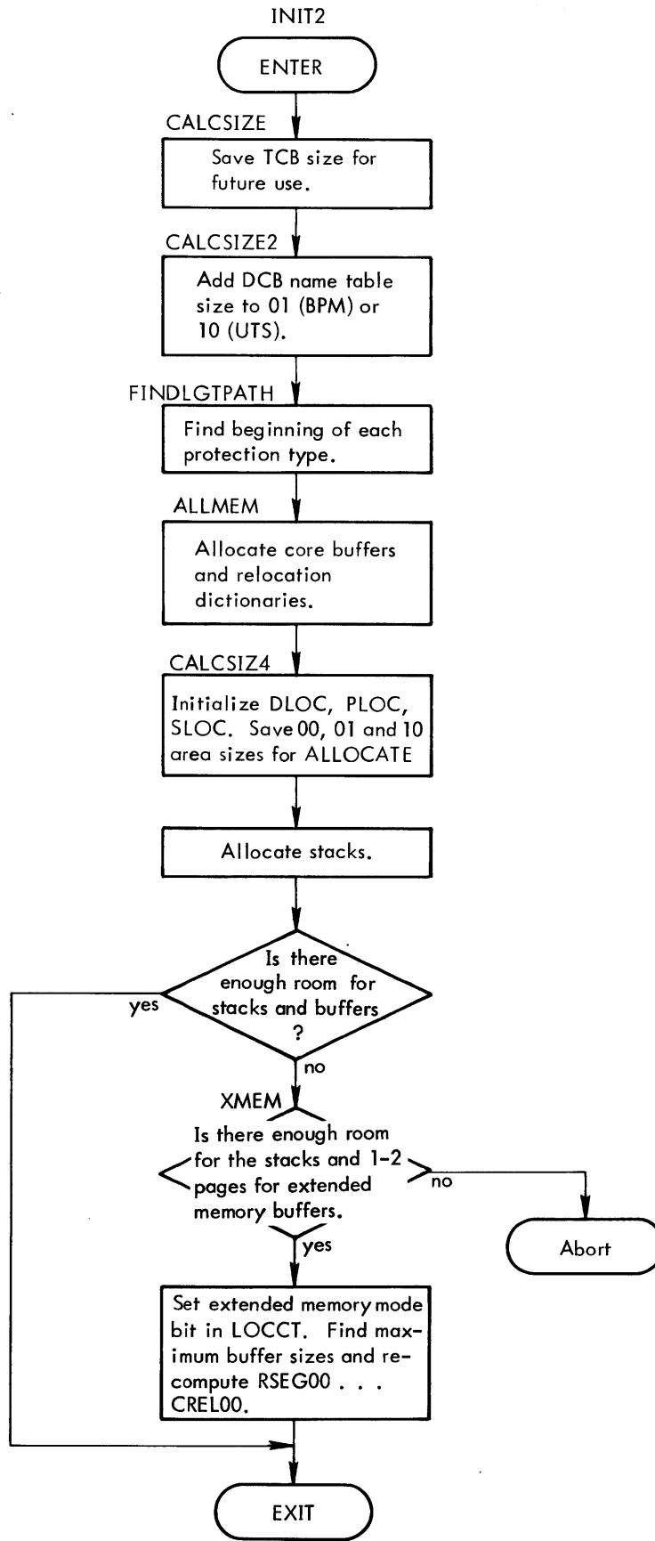
Figure 22. INIT2 Flow Chart
