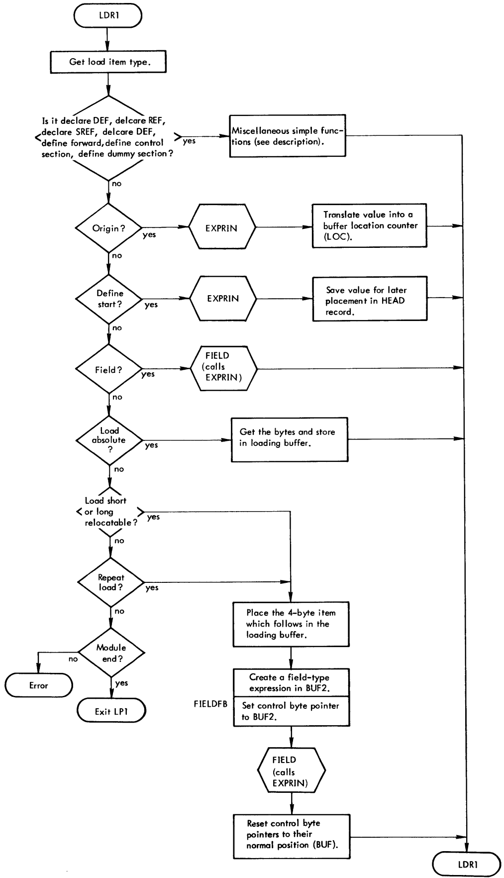
Figure 26. PASS2 Object Module Processor Flow Chart
