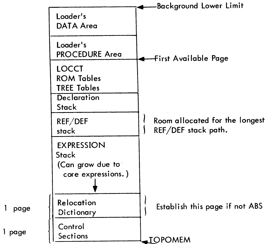
Figure 9a. How the Loader Uses Memory: Pass Two – Extended Memory Mode, Construction of Core Image Records
