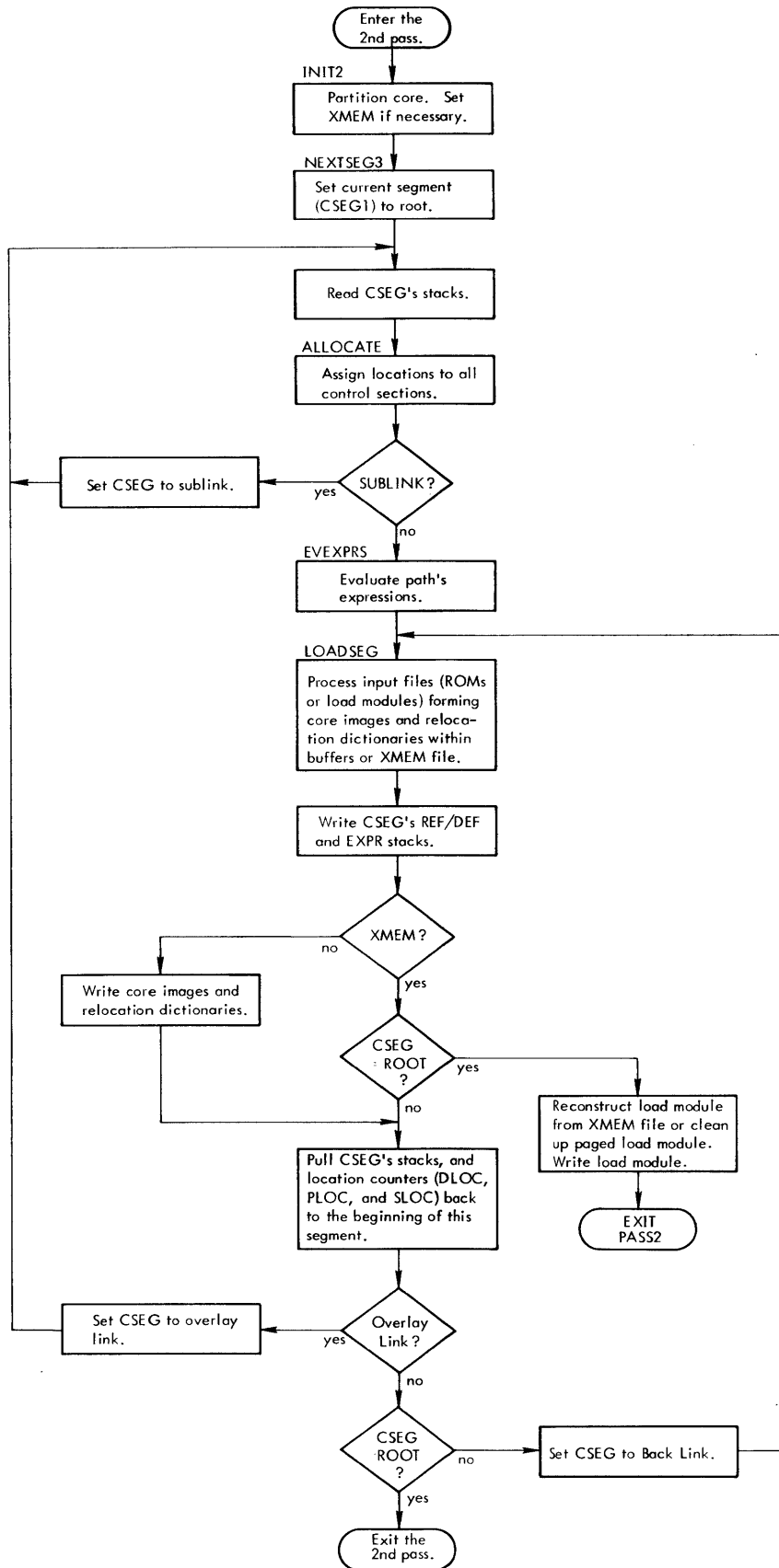
Figure 5. The Second Pass – General Flow
